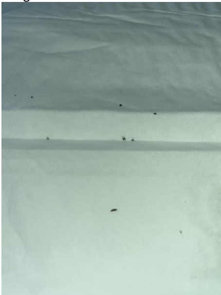
Laughlin circle
